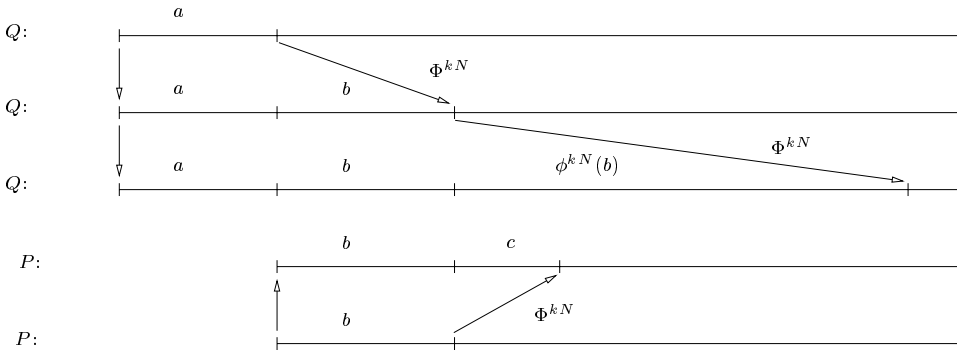
Figure 20.2. Proof of Corollary 20.3.
