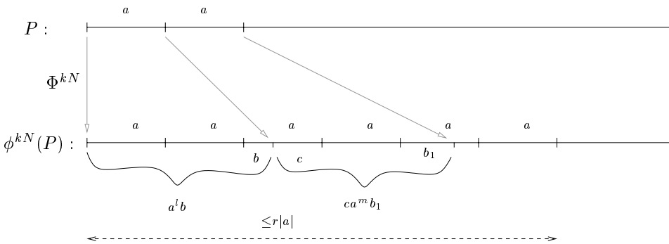
Figure 20.1. A priori estimate (Lemma 20.2).
