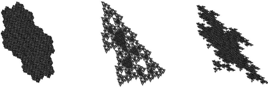
Figure 18.1. Rauzy Fractals for Tribonacci: 1 \mapsto 12, 2 \mapsto 13, 3 \mapsto 1 , and 1 \mapsto 12, 2 \mapsto 31, 3 \mapsto 1 , and 1 \mapsto 3211121, 2 \mapsto 231121, 3 \mapsto 3121 .
