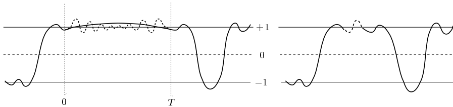
Fig. 5.1. The dashed curve represents the minimizer of J on the interval [0, T] from Theorem 4.1 which oscillates by Theorem 4.2. After pasting in the dashed curve, the function is clipped to restore the correct number of crossings. See Steps 1 and 5 in the proof of Theorem 5.6. A similar technique is used to prove Theorem 2.2
