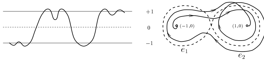
Fig. 1.1. A typical heteroclinic orbit with homotopy type e_1 e_2^2
