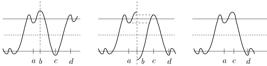
Fig. 7.1. An example of flipping and clipping in the proof of Lemma 7.4 (iii), Case 1
