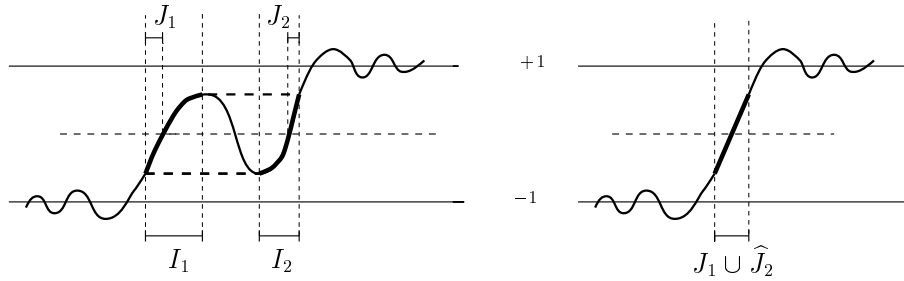
Fig. 3.1. A typical example of the clipping operation. As in Lemma 3.1, the intervals J_1 = [a_1, c_1] and J_2 = [c_2, b_2] are concatenated to [a_1, b_2 - c_2 + c_1] = [a_1, c_1] \cup [c_1, b_2 - c_2 + c_1] = J_1 \cup \widehat{J}_2
