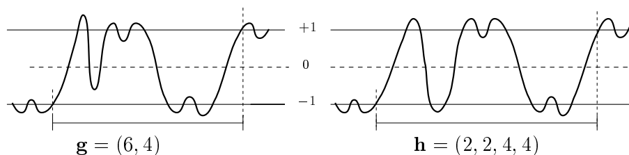
Fig. 2.1. (6, 4) \prec (2, 2, 4, 4) . The intervals pictured are the core intervals
